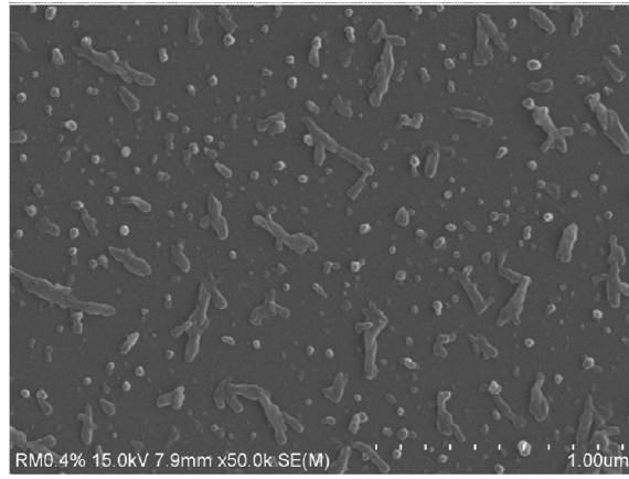
Figure 6. SEM image of surface in OCS cell with 0.4 wt% of RM concentration.
