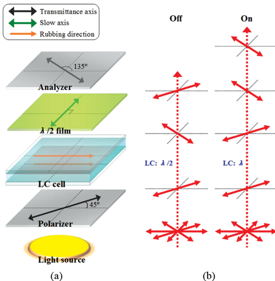
Figure 4. (a) Structure of OCS mode for normally black state and (b) variation of light polarization state through the OCS cell. (Figure appears in color online.)
